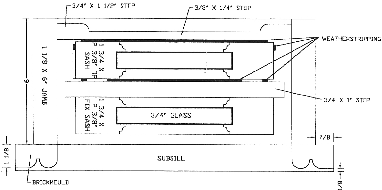
SINGLE HUNG JAMB SECTION (TOP VIEW)
