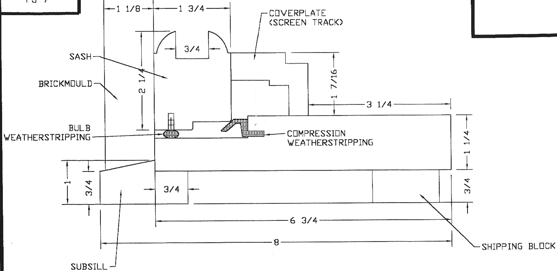
SILL PROFILE (CASEMENT WINDOW)
