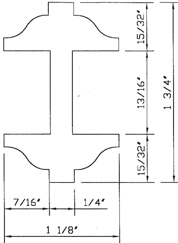
1 1/8" TRUE DIVIDED LIGHT (TDL) PROFILE
